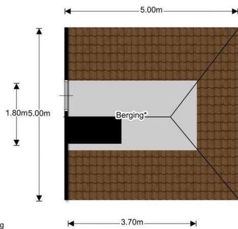
Vloring h nok ca. 2,30 m © Alex Housing
